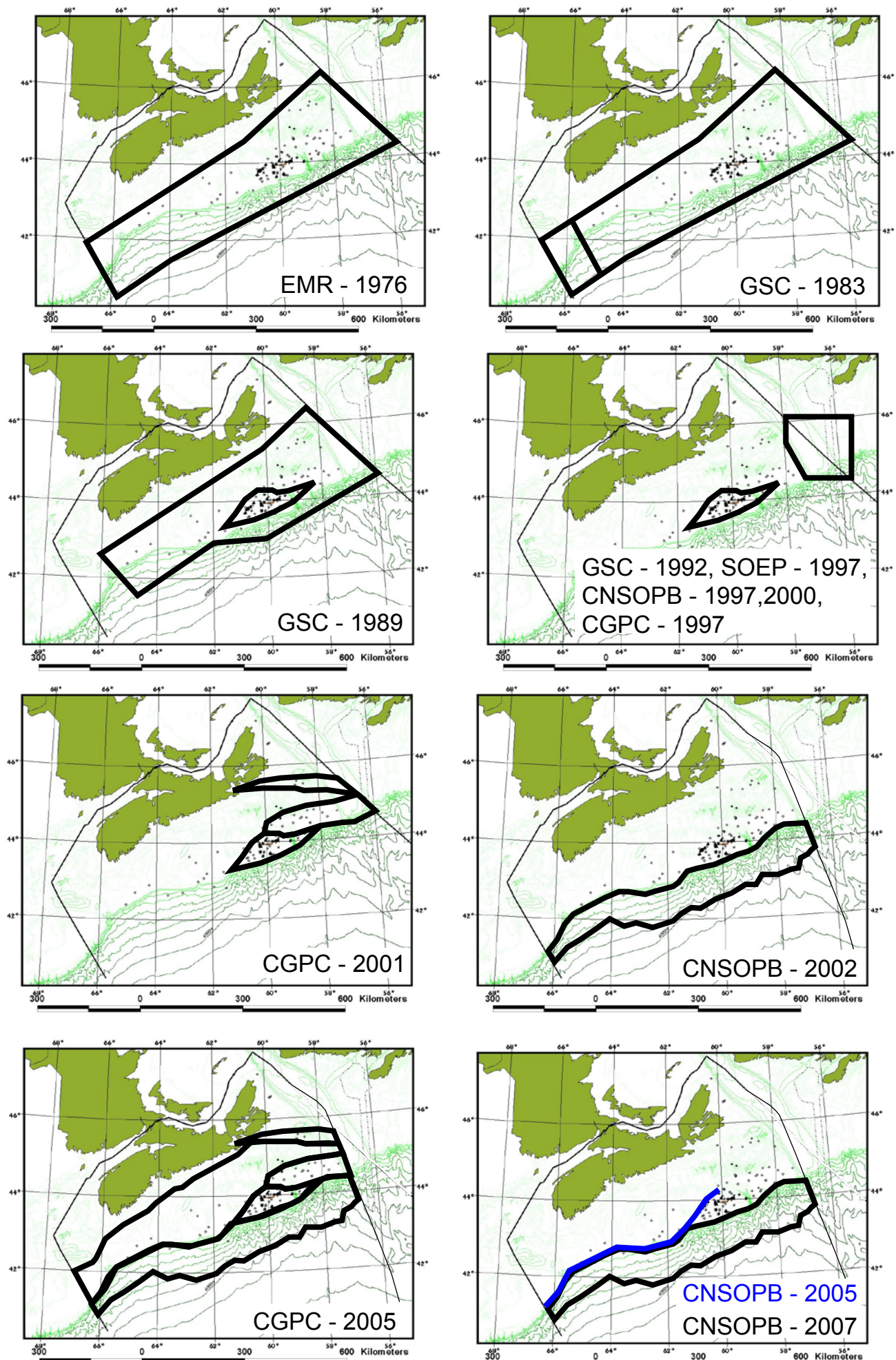
Figure 9: Areal distribution of historical petroleum resource and reserves assessments offshore Nova Scotia, 1976-2007.
